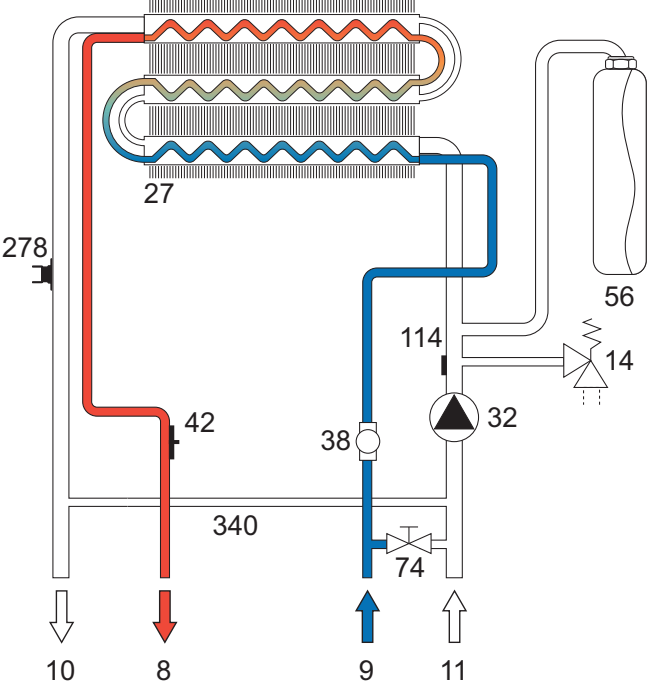
fig. 21 - DHW Circuit
