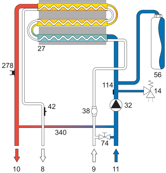
fig. 20 - Heating Circuit
