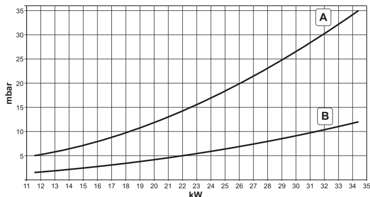
fig. 23 - Pressure - power diagram (DOMItech F 32 D)
